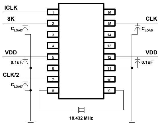
Figure 4. Test Circuit
