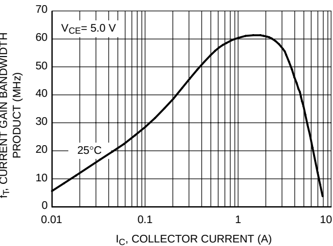
Figure 10. MJL0302A Current Gain Bandwidth Product
