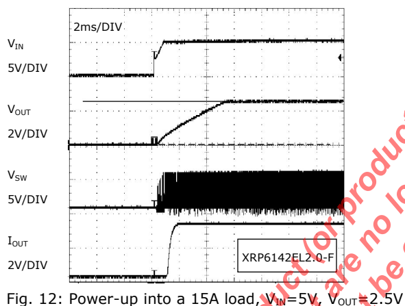
Fig. 12: Power-up into a 15A load, V_{IN}=5V , V_{OUT}=2.5V
