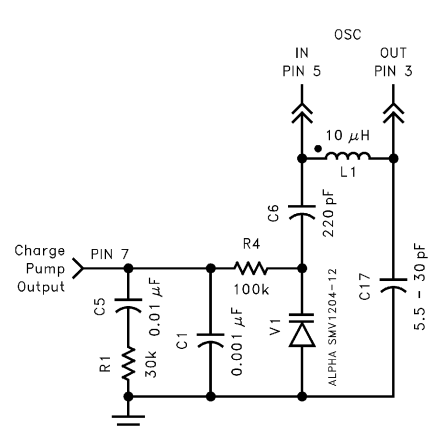
FIGURE 20. LC TANK
