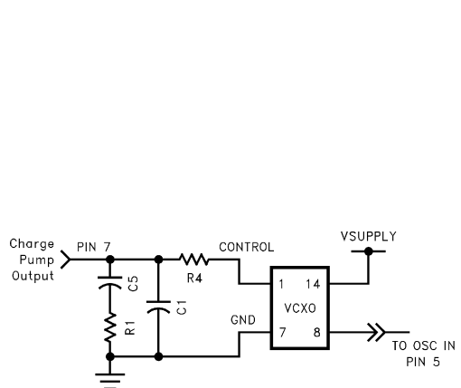
FIGURE 18. VCXO
