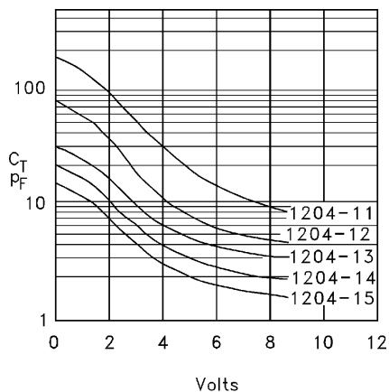
FIGURE 6. TYPICAL VARACTOR
