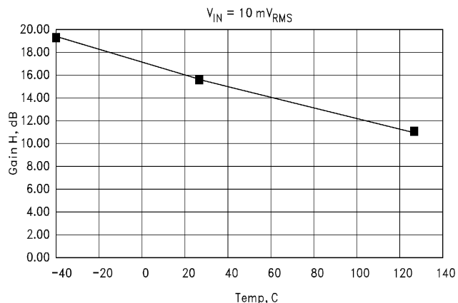
FIGURE 5. EL4584 OSC GAIN @ 20MHz vs TEMPERATURE
