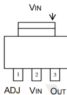
SOT-223-3 (TOP VIEW)
