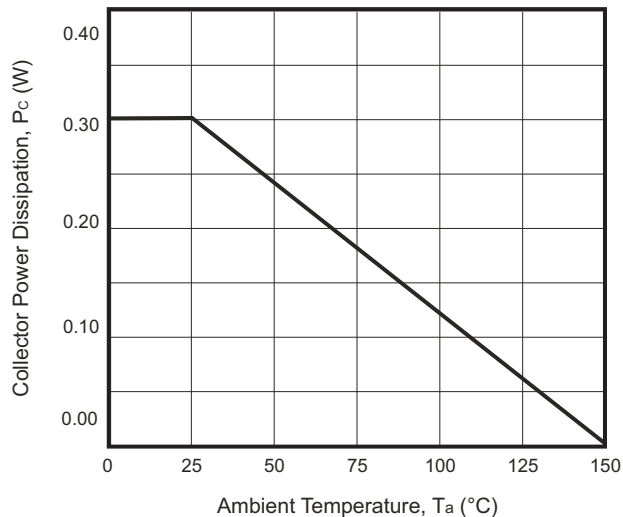
Fig.8 - P_C - T_a
