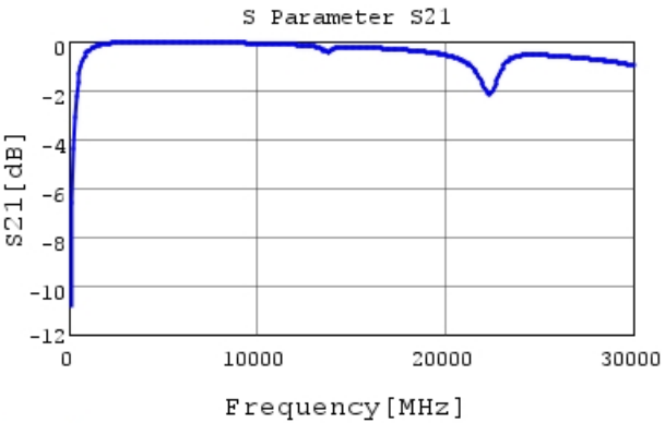
GJM0335C1E4R8WB01 S21 DCOV, 25degC
