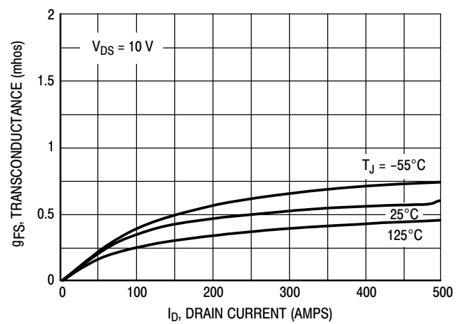
Figure 8. Transconductance
