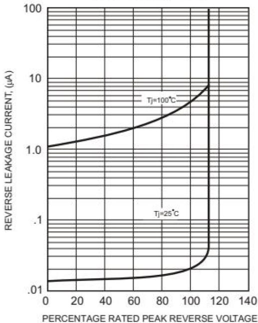
FIG.3 - TYPICAL REVERSE
