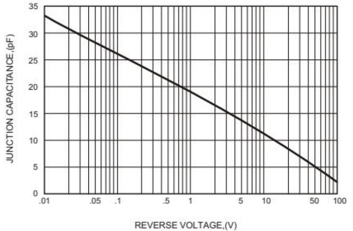
FIG.5-TYPICAL JUNCTION CAPACITANCE
