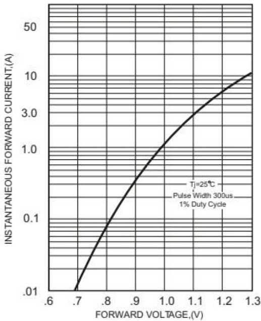
FIG.1-TYPICAL FORWARD
