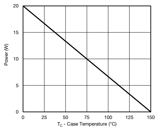
Power, Junction-to-Case
