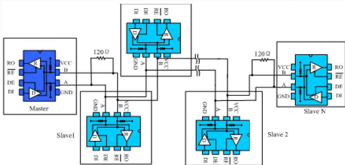
Fig. 10 Hand-in-hand type RS485 half-duplex communication network
