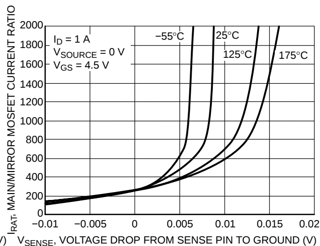
Figure 12. Current Ratio versus V_{SENSE}
