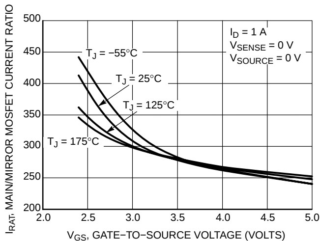
Figure 10. Current Ratio versus V_{GS}
