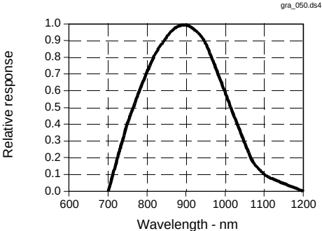
Fig. 5 Spectral Responsivity
