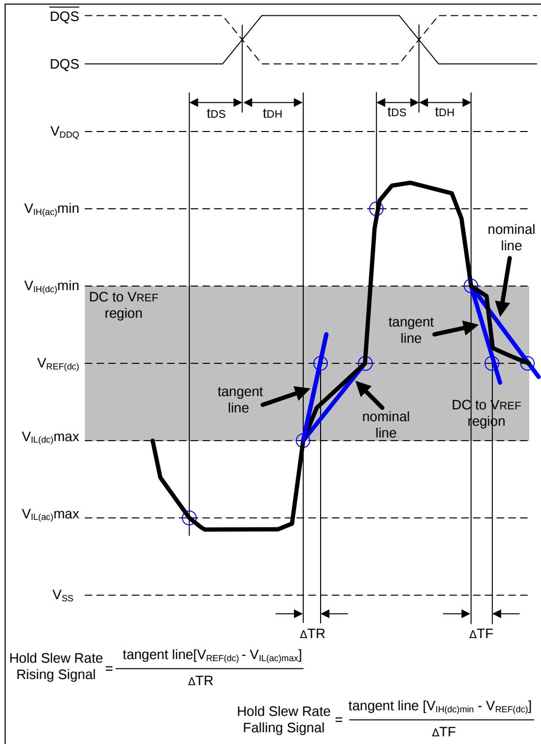
Figure 27 —Illustration tangent line for t_{DH} (differential \text{DQS}, \overline{\text{DQS}} )
