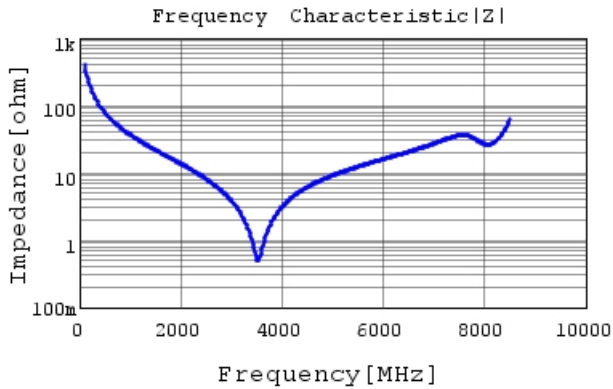
GRM1885C2A4R0WA01 |Z| DCOV, 25degC
