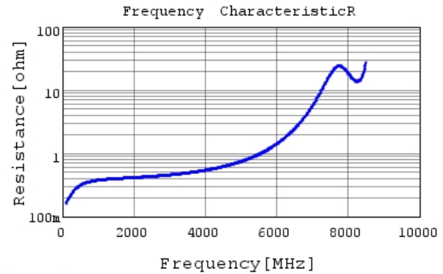
GRM1885C2A4R0WA01 R DCOV, 25degC
