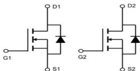
SOP-8
