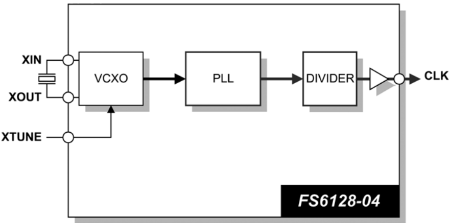
Figure 2: Block Diagram
