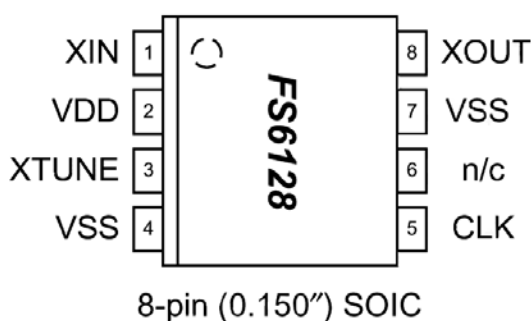
Figure 1: Pin Configuration
