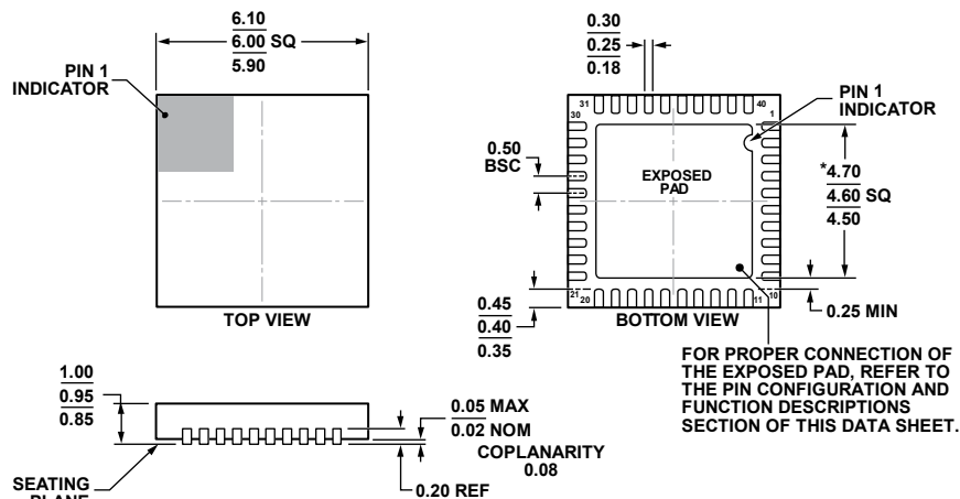
Figure 51. 40-Lead Lead Frame Chip Scale Package [LFCSP]
