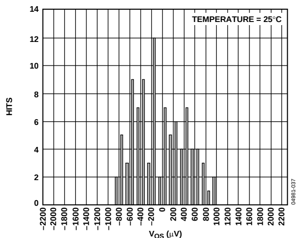
Figure 19. V_{OS} Distribution, MSOP, Temperature = 25°C
