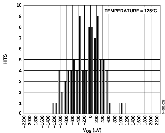
Figure 20. V_{OS} Distribution, MSOP, Temperature = 125°C
