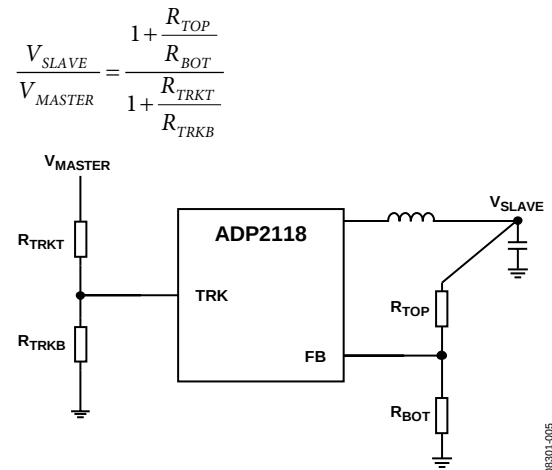
Figure 42. Voltage Tracking
