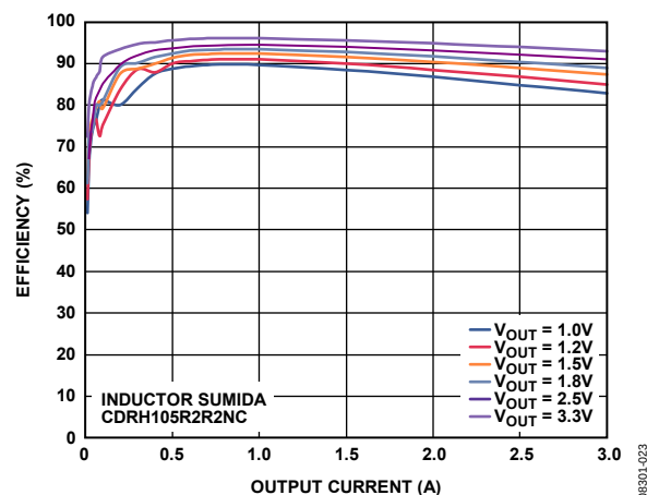
Figure 13. Efficiency (600 kHz, V_{IN} = 5 V, PFM) vs. Output Current
