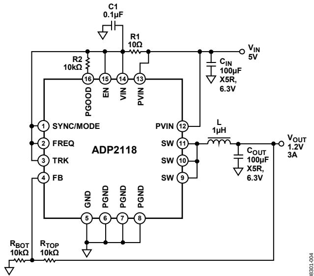
Figure 41. Application Circuit
