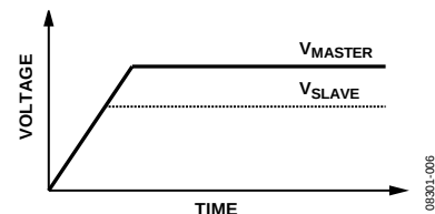
Figure 43. Coincident Tracking
