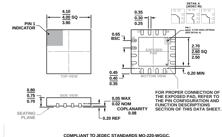
Figure 50. 16-Lead Lead Frame Chip Scale Package [LFCSP] 4 mm × 4 mm Body and 0.75 mm Package Height (CP-16-17)
