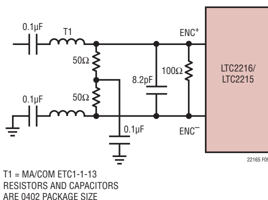
Figure 9. Balun-Driven Encode
