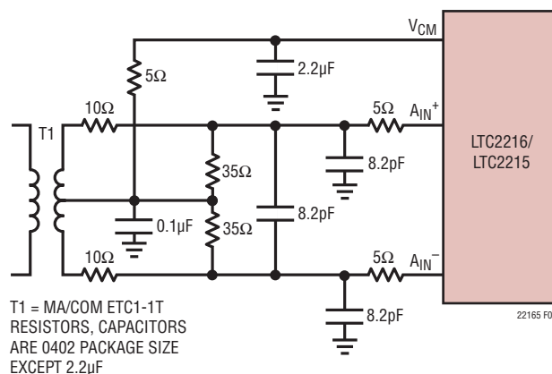
Figure 3. Single-Ended to Differential Conversion Using a Transformer. Recommended for Input Frequencies from 5\text{MHz} to 100\text{MHz}
