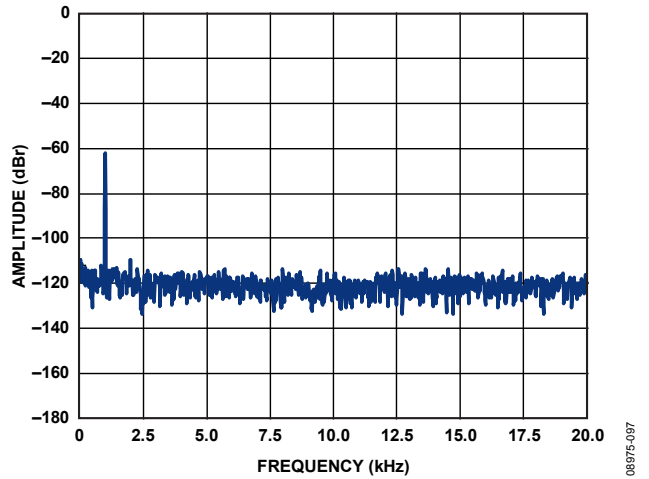
Figure 66. FFT, -60 dBFS, Digital In → Digital Out
