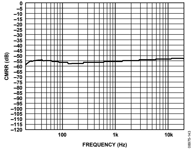
Figure 64. CMRR vs. Frequency, Analog In → Digital Out, PGA Gain = 0 dB
