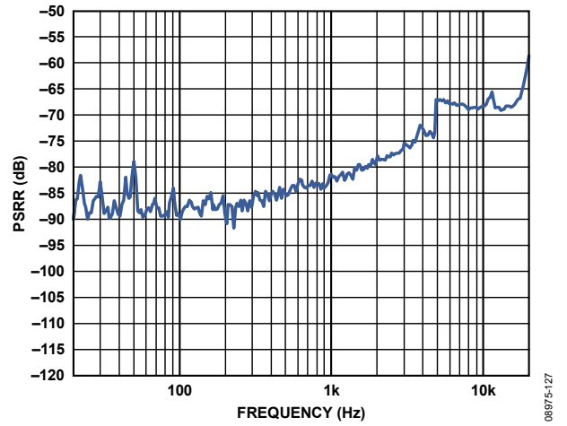
Figure 65. PSRR vs. Frequency Ripple on AVDD, Analog In → Digital Out, PGA Gain = 0 dB
