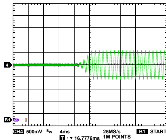
Figure 77. Turn On Headphone Out
