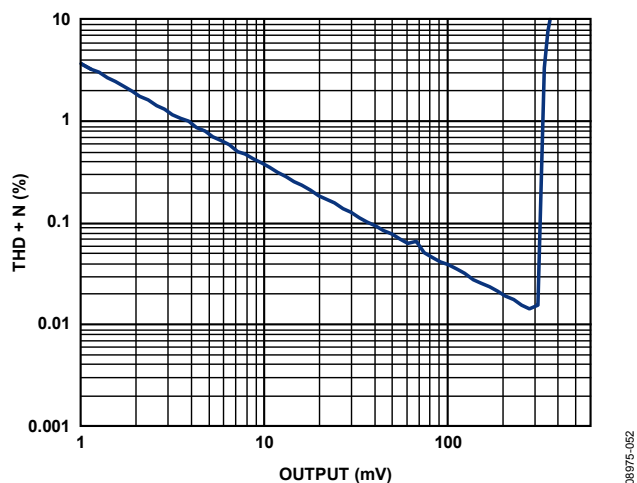
Figure 9. THD + N vs. Output Level, Analog In → Line Out
