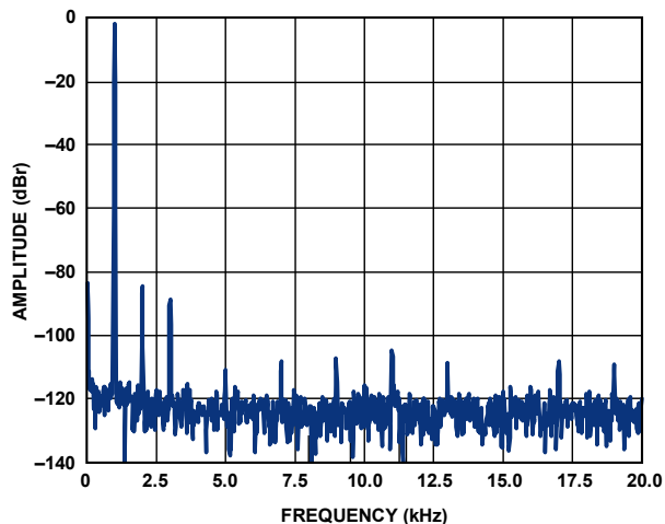
Figure 46. FFT, -1 dBFS, 16 \Omega , Digital In \rightarrow Headphone Out
