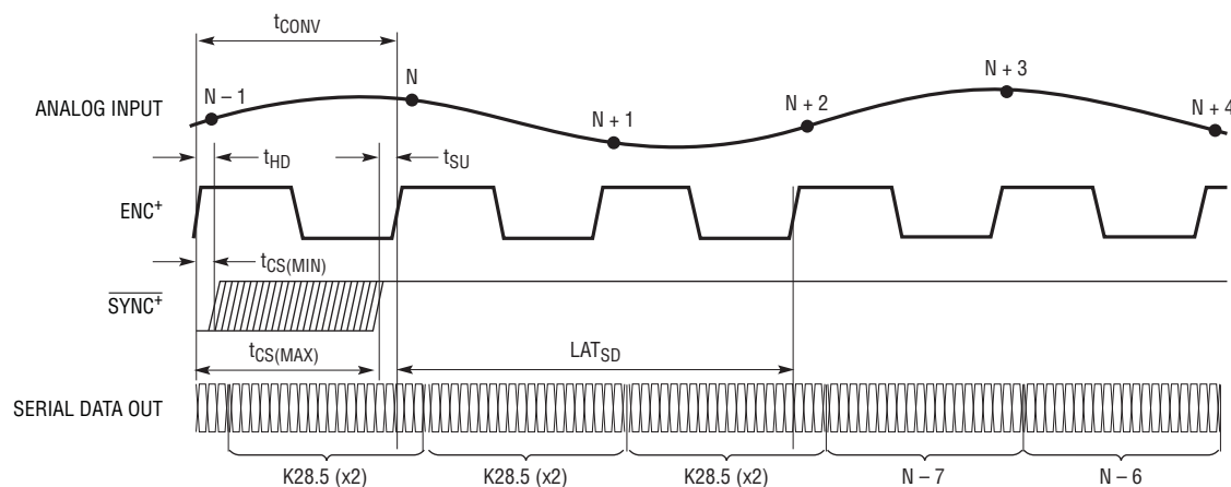
Figure 14b. \overline{\text{SYNC}}^+ High Transition to Data Output Timing (ISMODE is Low)
