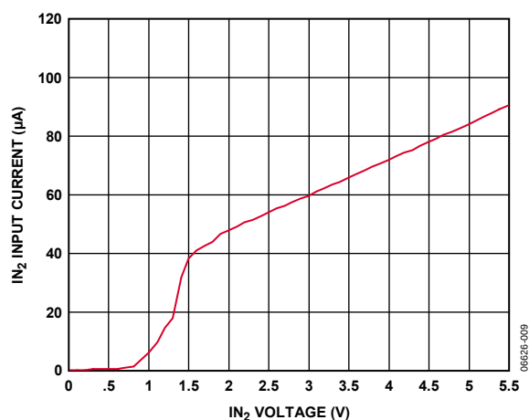
Figure 5. IN_2 Input Current vs. IN_2 Voltage
