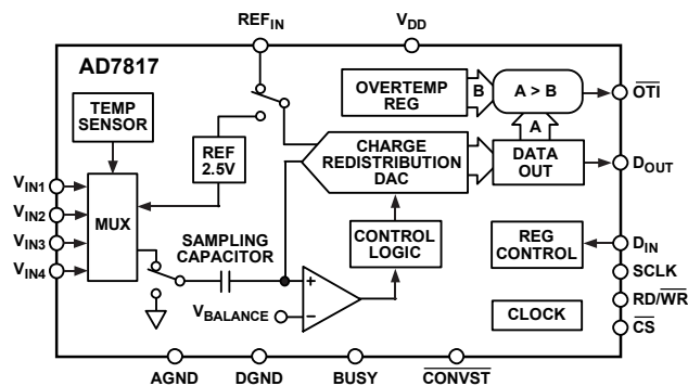
Figure 1. AD7817 Functional Block Diagram
