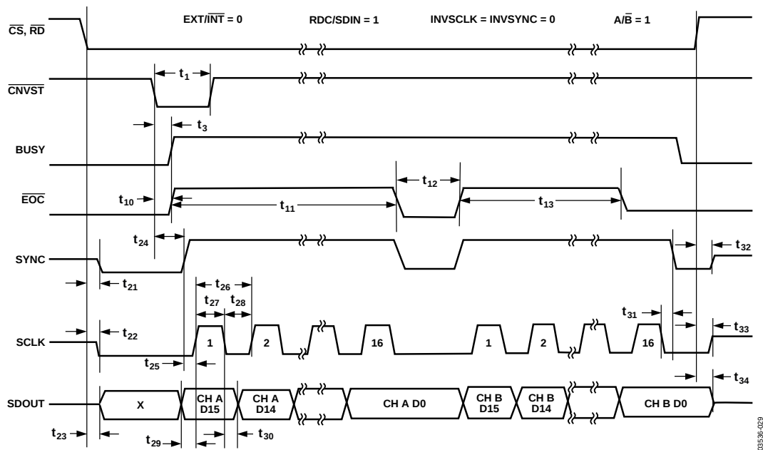
Figure 30. Master Serial Data Timing for Reading (Read Previous Conversion During Convert)
