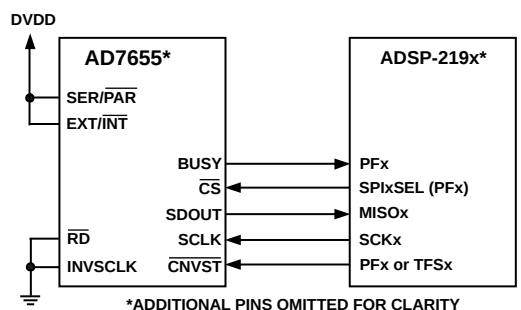
Figure 34. Interfacing the AD7655 to SPI Interface
