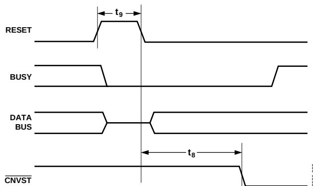
Figure 23. Reset Timing
