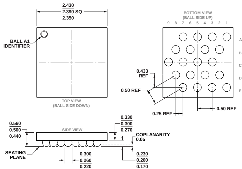
Figure 47. 20-Ball Wafer Level Chip Scale Package [WLCSP]
