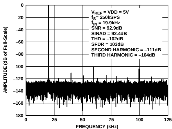
Figure 10. 20 kHz FFT, V_{REF} = V_{DD} = 5\text{ V}
