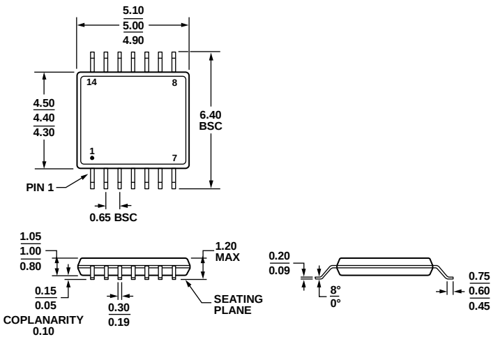
COMPLIANT TO JEDEC STANDARDS MO-153-AB-1 Figure 61. 14-Lead Thin Shrink Small Outline Package [TSSOP] (RU-14) Dimensions shown in millimeters
