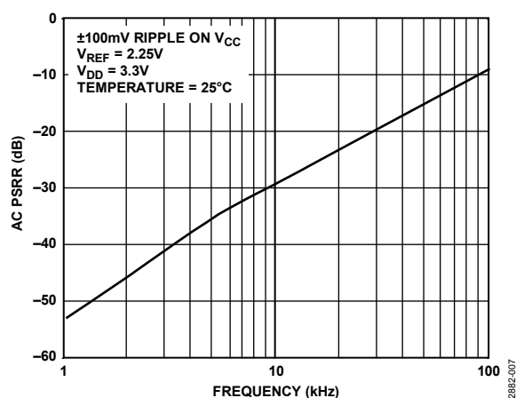
Figure 8. PSRR vs. Supply Ripple Frequency
