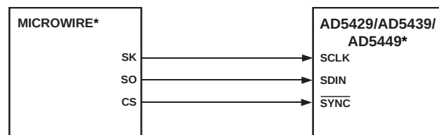
Figure 54. MICROWIRE-to-AD5429/AD5439/AD5449 Interface
