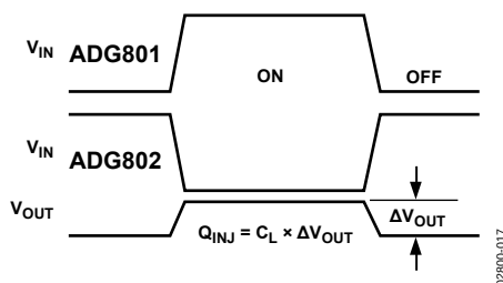
Figure 17. Charge Injection
