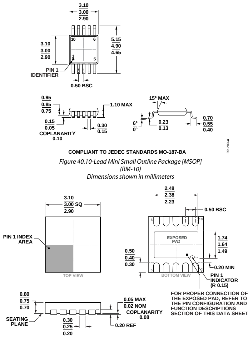
Figure 41. 10-Lead Lead Frame Chip Scale Package [LFCSP_WD] 3 mm × 3 mm Body, Very Very Thin, Dual Lead (CP-10-9) Dimensions shown in millimeters
