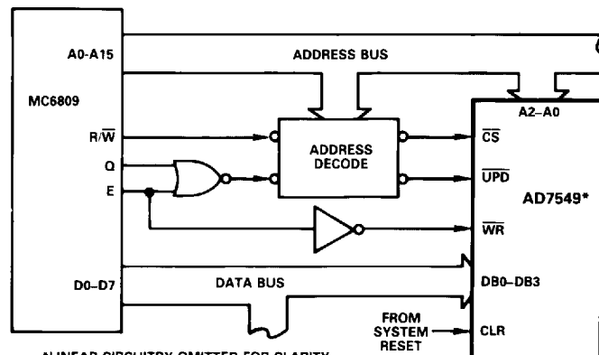
Figure 8. AD7549-MC6809 Interface
