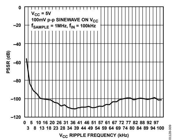
Figure 9. Typical Power Supply Rejection Ratio (PSRR)
