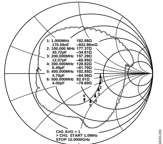
Figure 44. Different Input Return Loss
