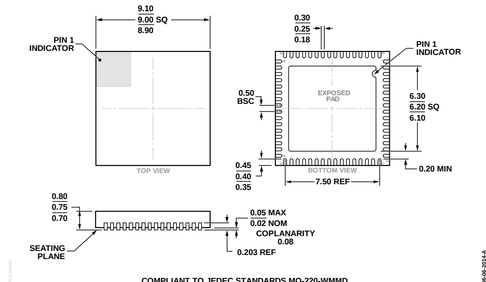
COMPLIANT TO JEDEC STANDARDS MO-220-WMMD Figure 118. 64-Lead Lead Frame Chip Scale Package [LFCSP] 9 mm × 9 mm Body and 0.75 mm Package Height (CP-64-17) Dimensions shown in millimeters
