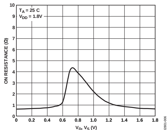
Figure 6. On Resistance vs. V_D , V_S
