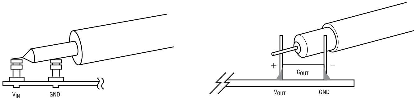
Figure 2. Measuring Input or Output Ripple Across Terminals or Directly Across Bulk Capacitor
