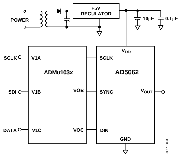
Figure 44. AD5662 with a Galvanically Isolated Interface
