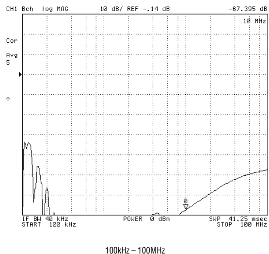
Figure 3. Typical Adjacent-Channel Crosstalk
