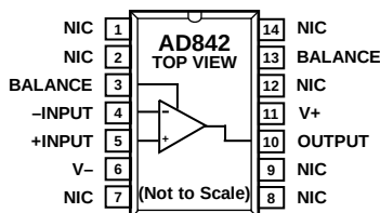
Figure 1. PDIP (N-14) and CERDIP (Q-14)
