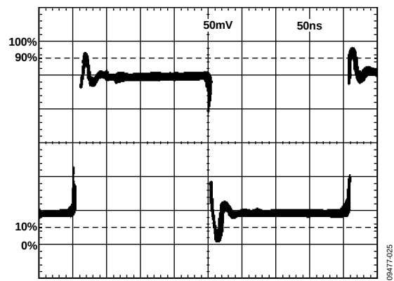
Figure 26. Noninverting Small Signal Pulse Response (see Figure 27)
