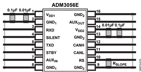
Figure 26. Recommended Printed Circuit Board Layout
