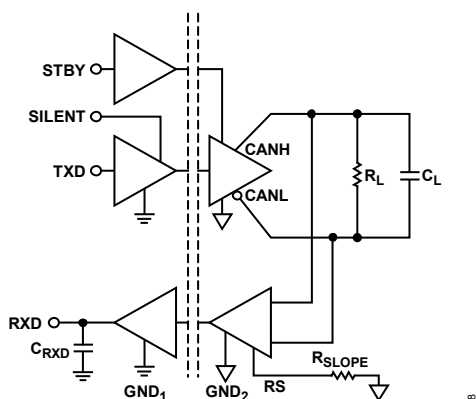
Figure 23. Switching Characteristics Measurements
