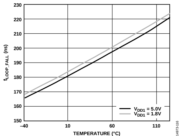
Figure 16. t_{LOOP\_FALL} vs. Temperature ( R_{SLOPE} = 47\ k\Omega )
