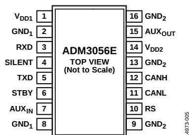
Figure 7. Pin Configuration
