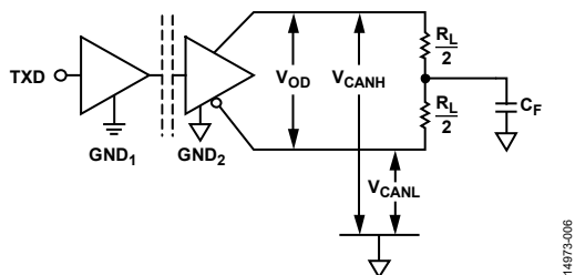
Figure 21. Driver Voltage Measurement
