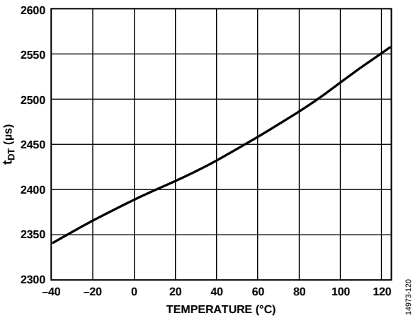
Figure 20. t DT vs. Temperature
