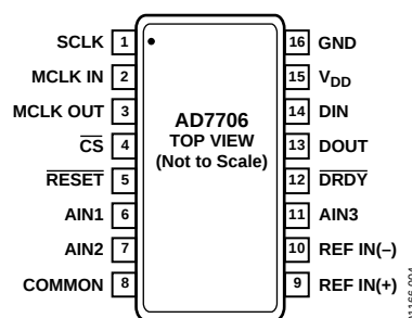
Figure 4. AD7706 Pin Configuration
