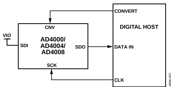
Figure 52. \overline{\text{CS}} Mode, 3-Wire Without Busy Indicator Connection Diagram (SDI High)
