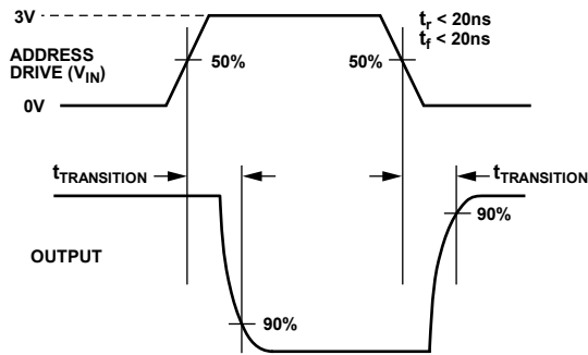
Figure 15. Address to Output Switching Times, t_{\text{TRANSITION}}
