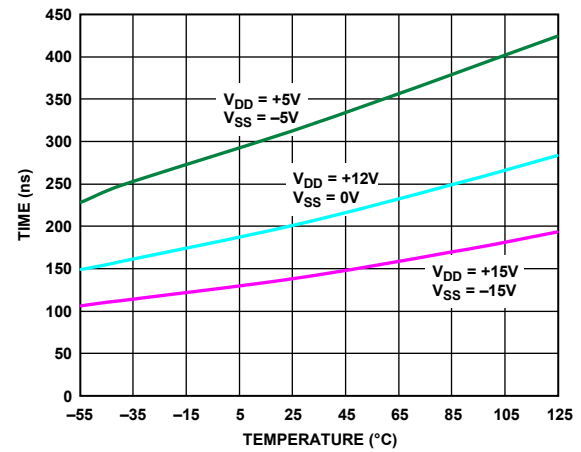
Figure 7. Transition Time vs. Temperature
