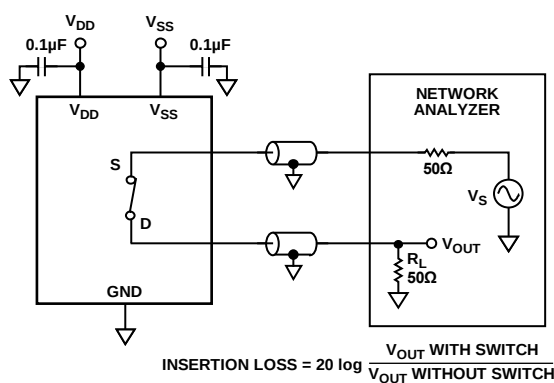
Figure 21. Insertion Loss
