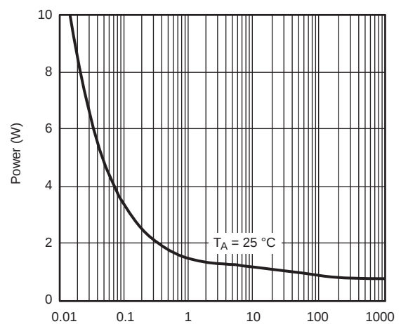
T_A = 25\text{ °C} Single Pulse Power
