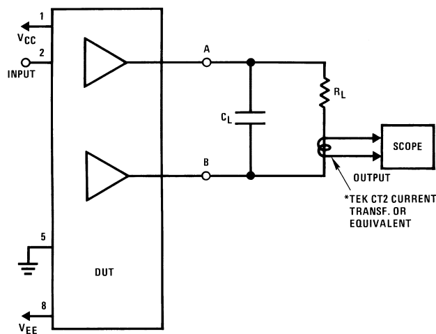
Figure 3. Differential Connection
