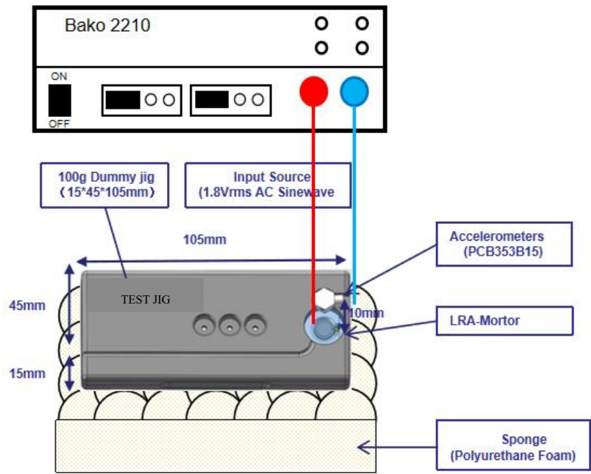
An Example of Measurement Method of Figure 2 测试方法 图 2
