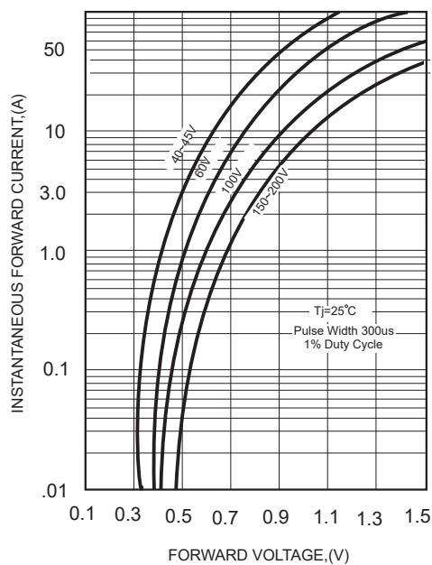
FIG.2-TYPICAL FORWARD CHARACTERISTICS
