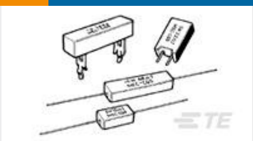
TE Part #2-1623789-6 SQM7 390R 5% (WIRE)
