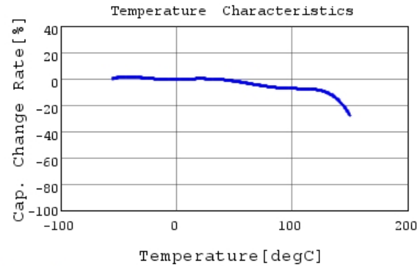
GCJ188L81H472MA01 C-Temp. capchange, DC0.0V,
