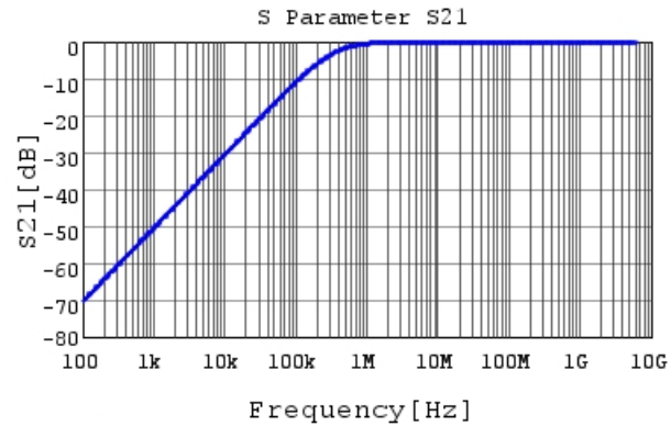
GCJ188L81H472MA01 S21 DC0V, 25degC
